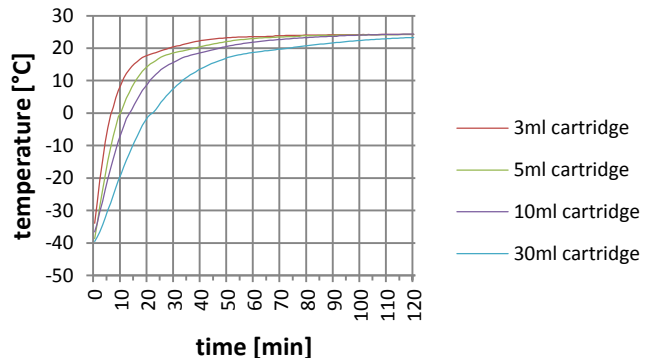
Thawing curve -40°C
