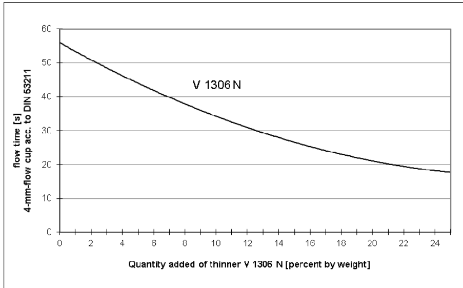
Fig. 1: Viscosity depending on the quantity of thinner added to conformal coating ELPEGUARD® SL 1306 N at 20 °C
