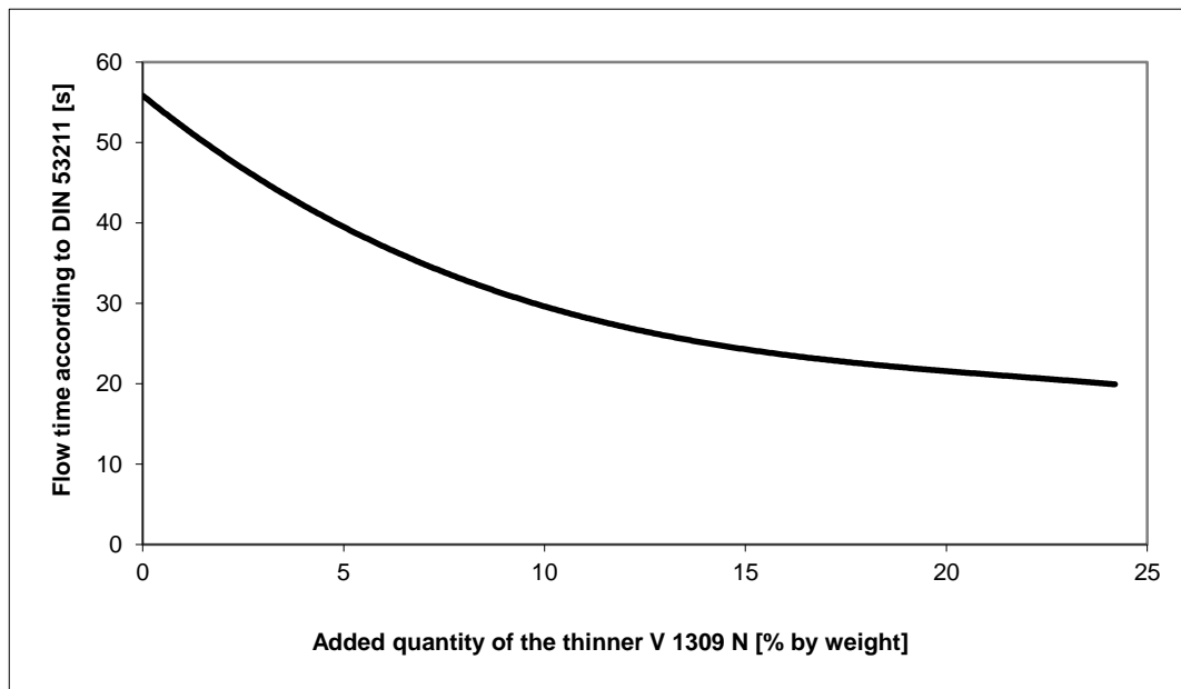
Fig. 1: Viscosity depending on the quantity of thinner added to conformal coating ELPEGUARD® SL 1309 N-FLZ at 20 °C [68 °F]
