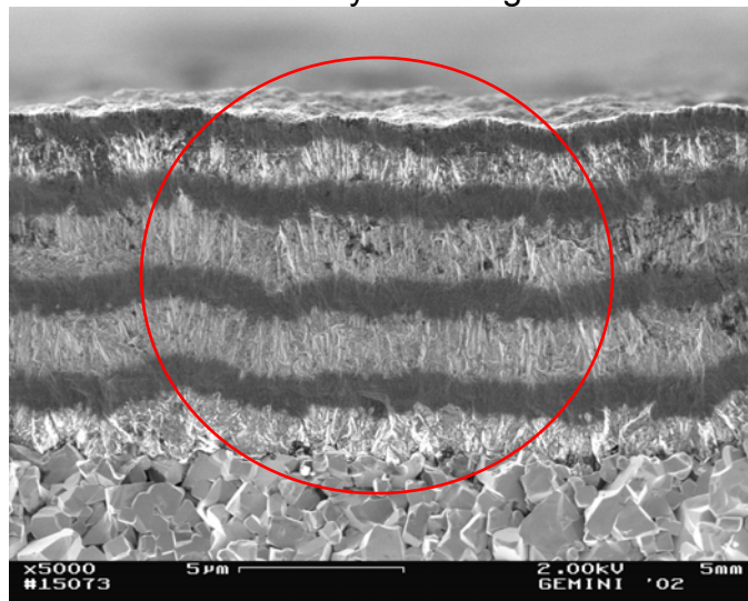
Multilayer coating
